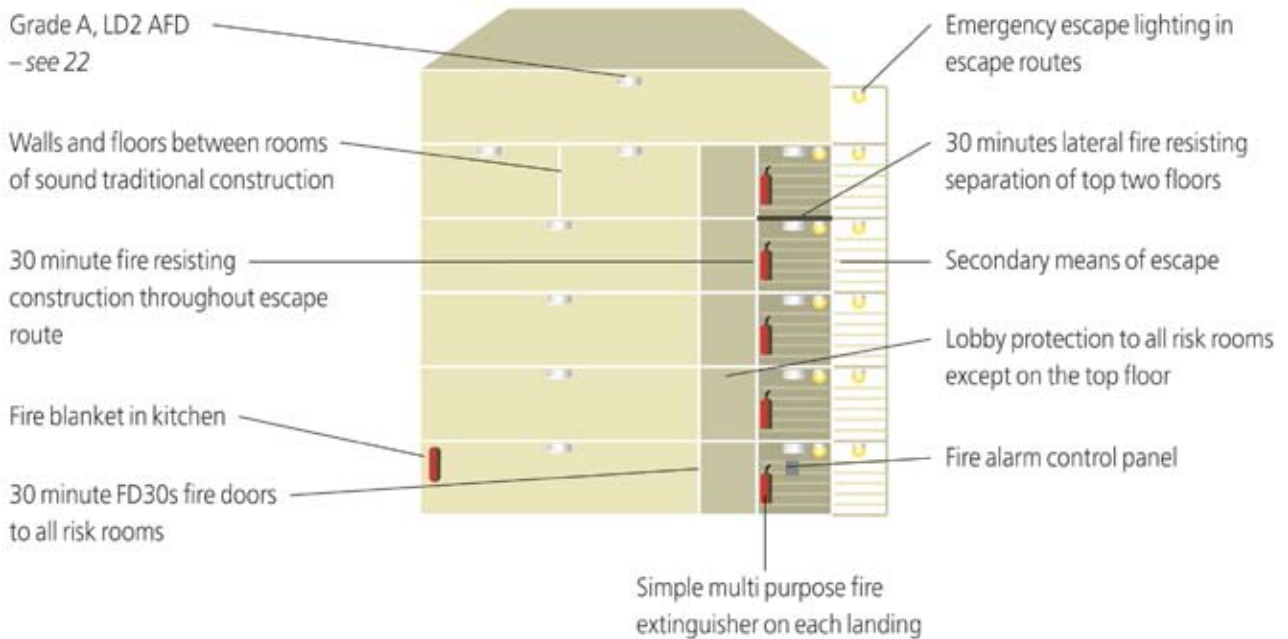
figure D6: shared house of six storeys
